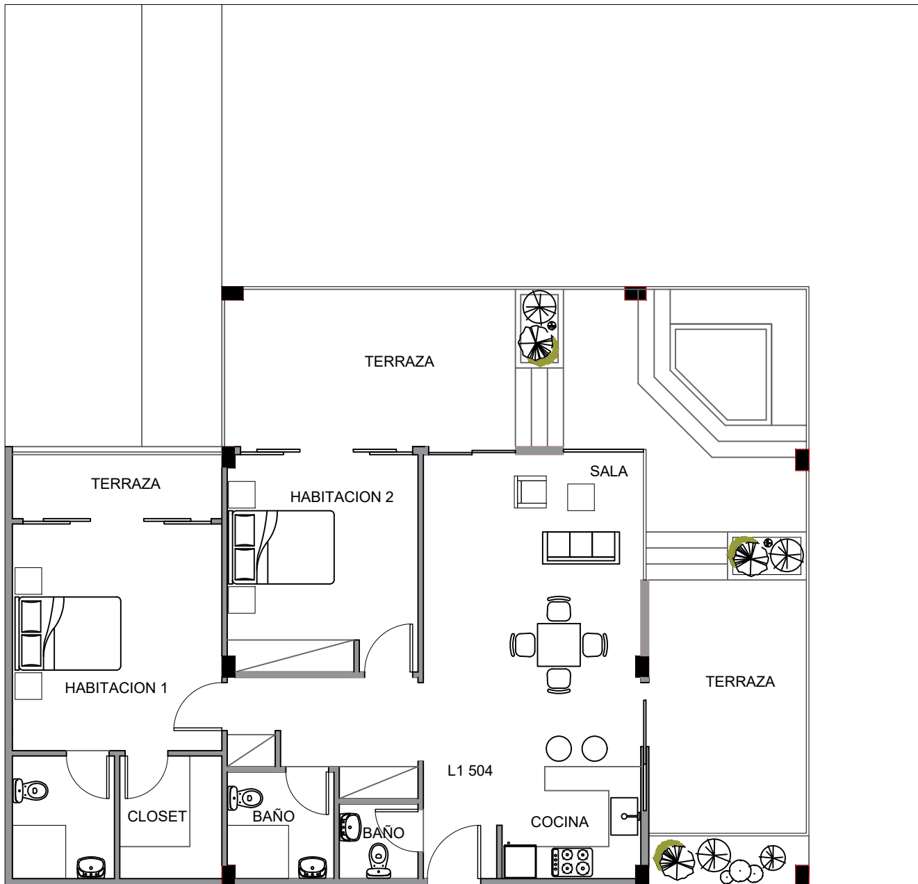
PLANO APTO L1 504 MT2: 155.51
