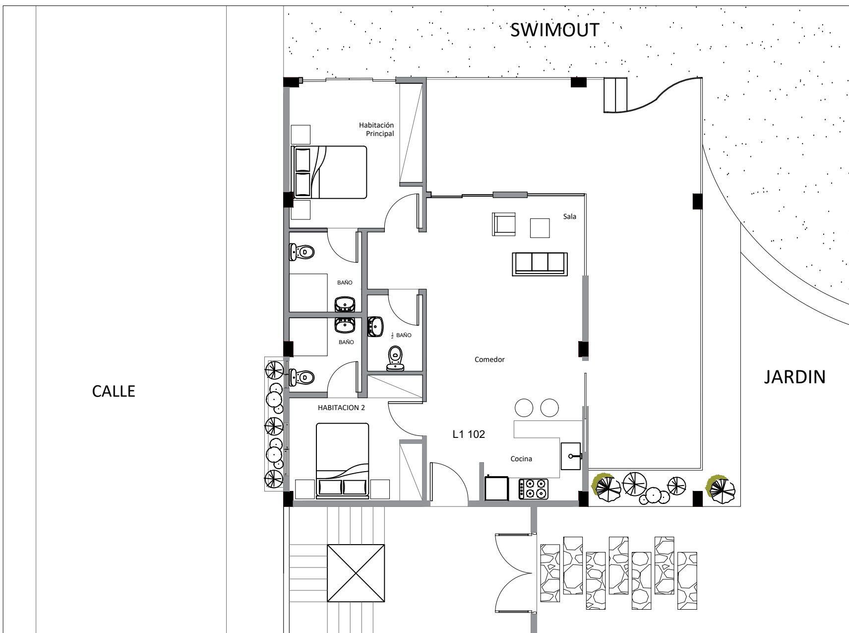
PLANO APTO L1 102 MT2: 120.90
